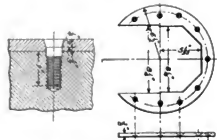
Figs. 3422-3424. Box Liner.
